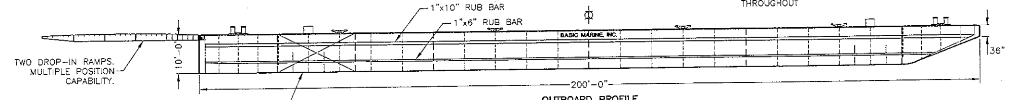
OUTBOARD PROFILE
