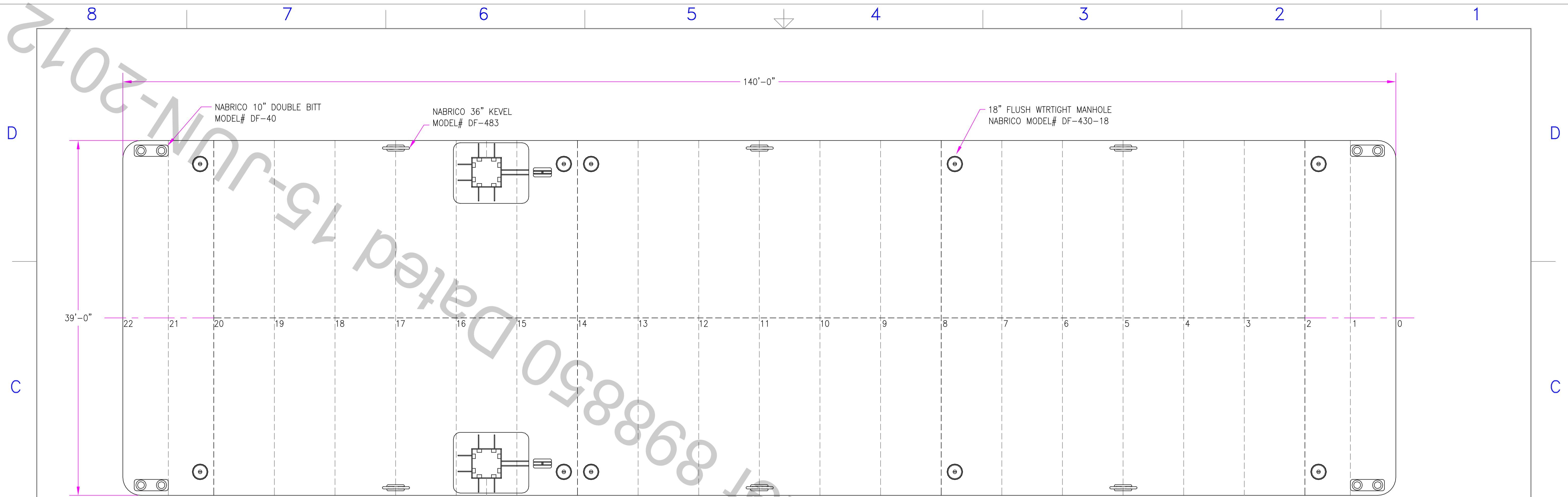
GENERAL ARRANGEMENT — HOLD PLAN VIEW
