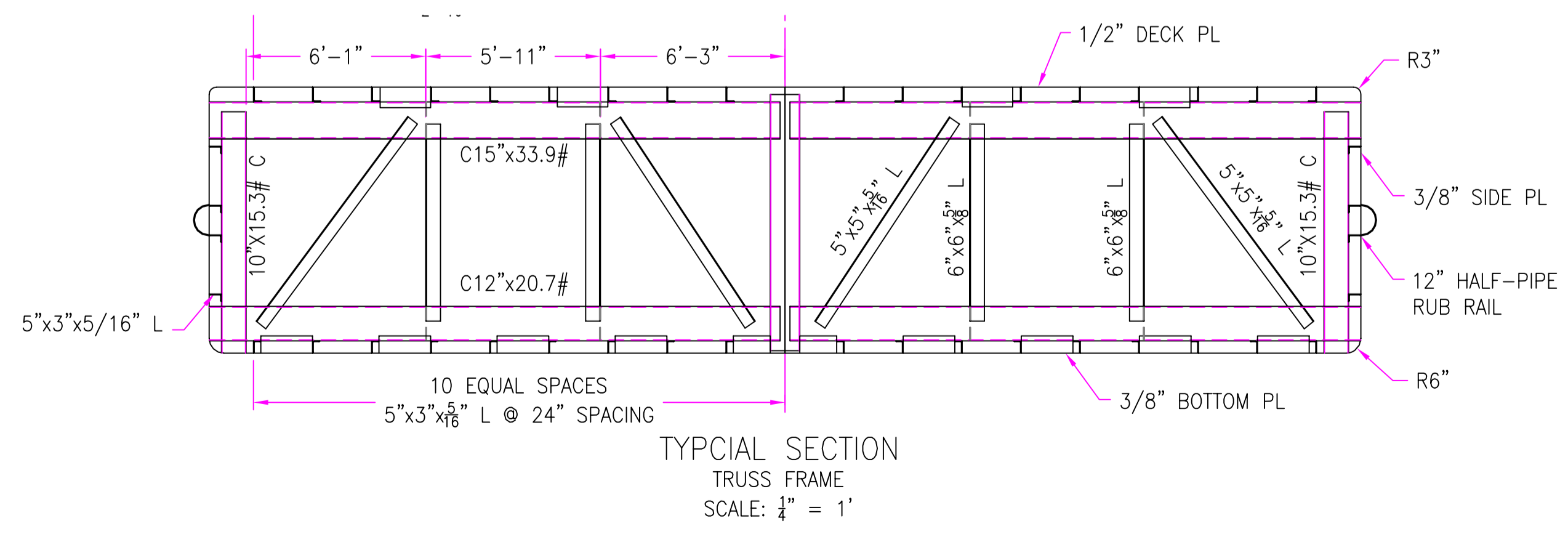
OUTBOARD PROFILE
