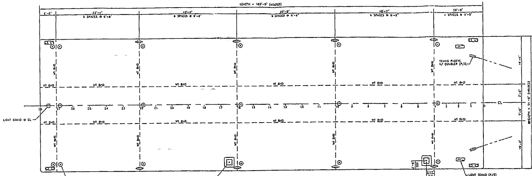
DECK ARRANGEMENT
